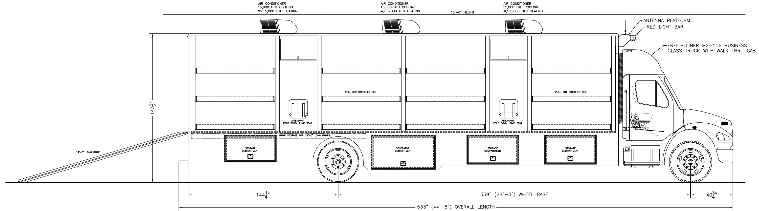
INTERIOR ROAD SIDE LAYOUT
